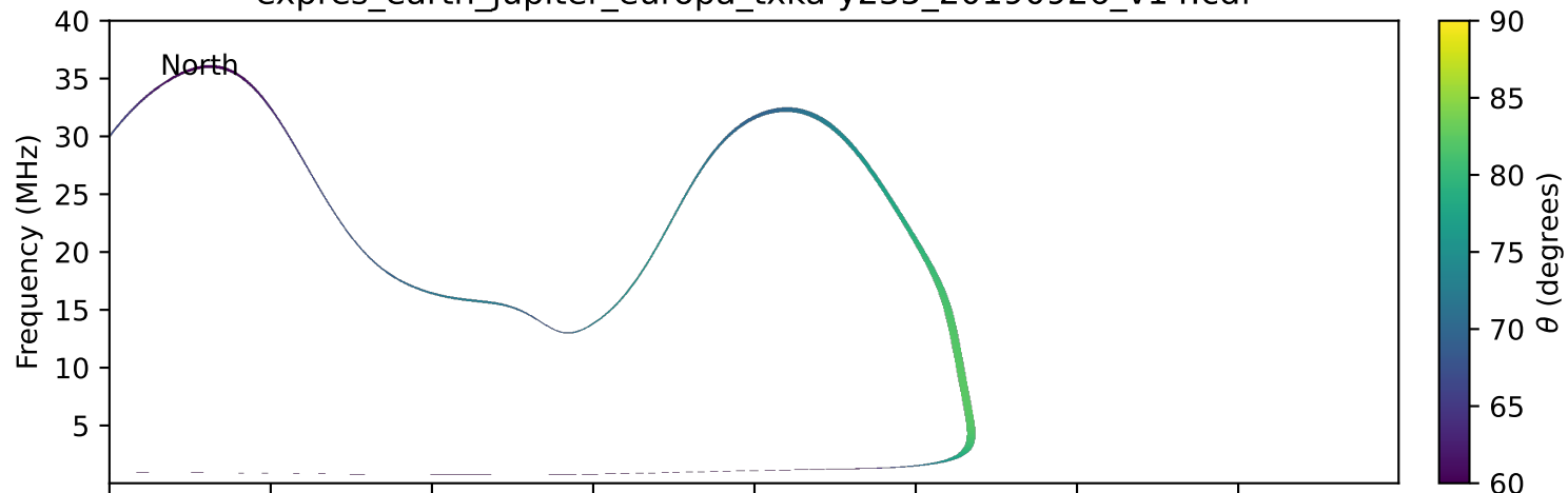
expres_earth_jupiter_europa_txka-y235_20190926_v14.cdf
