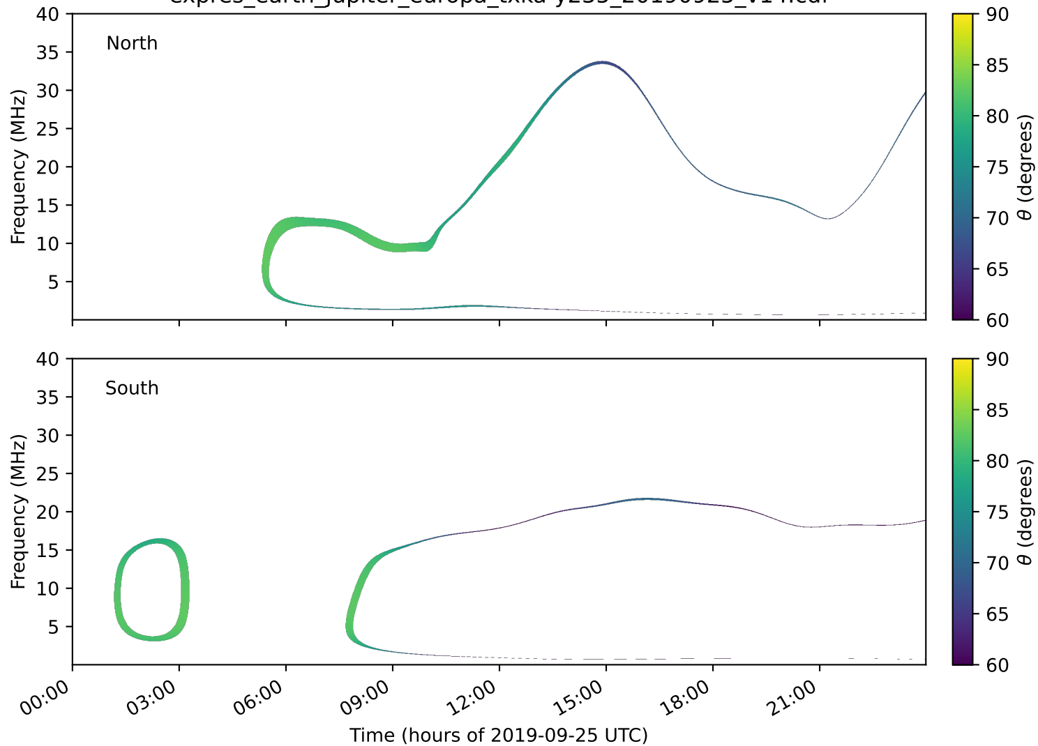
expres_earth_jupiter_europa_txka-y235_20190925_v14.cdf
