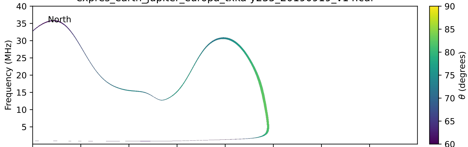
expres_earth_jupiter_europa_txka-y235_20190919_v14.cdf
