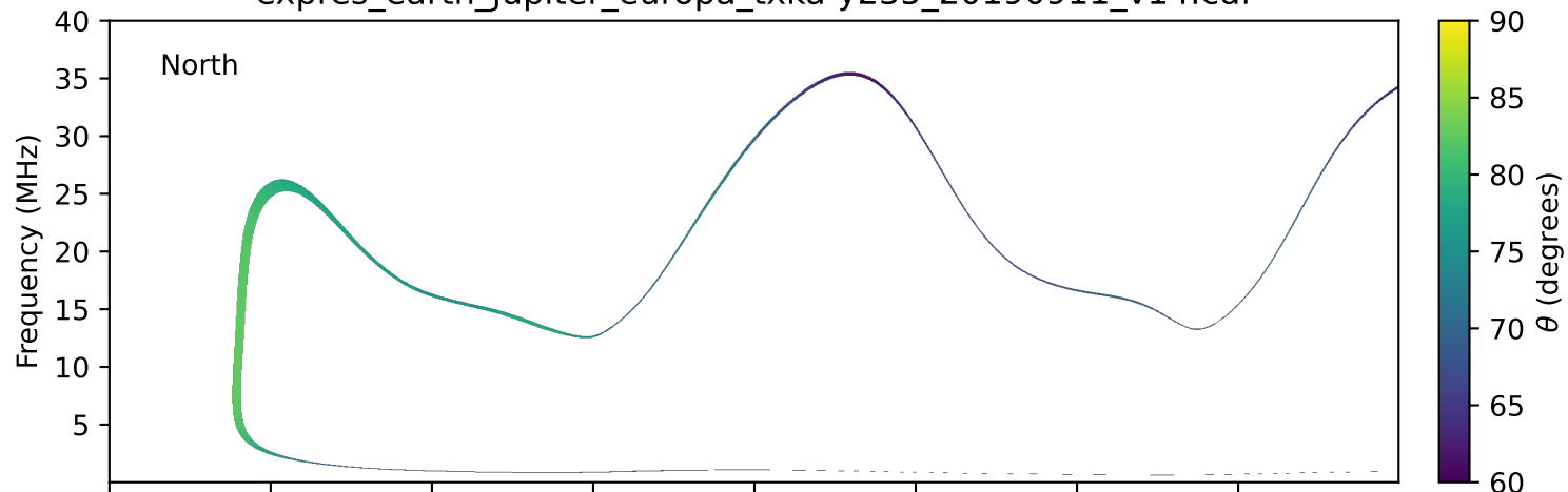
expres_earth_jupiter_europa_txka-y235_20190911_v14.cdf
