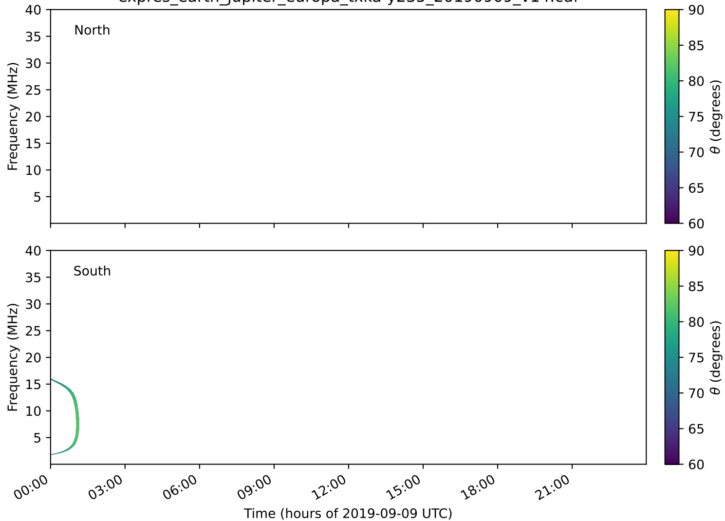
expres_earth_jupiter_europa_txka-y235_20190909_v14.cdf
