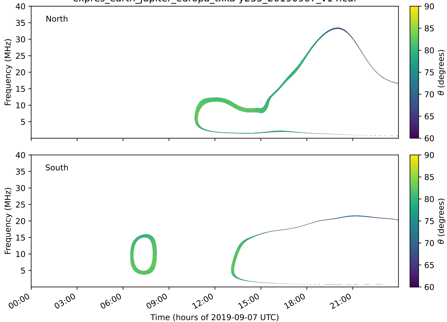
expres_earth_jupiter_europa_txka-y235_20190907_v14.cdf
