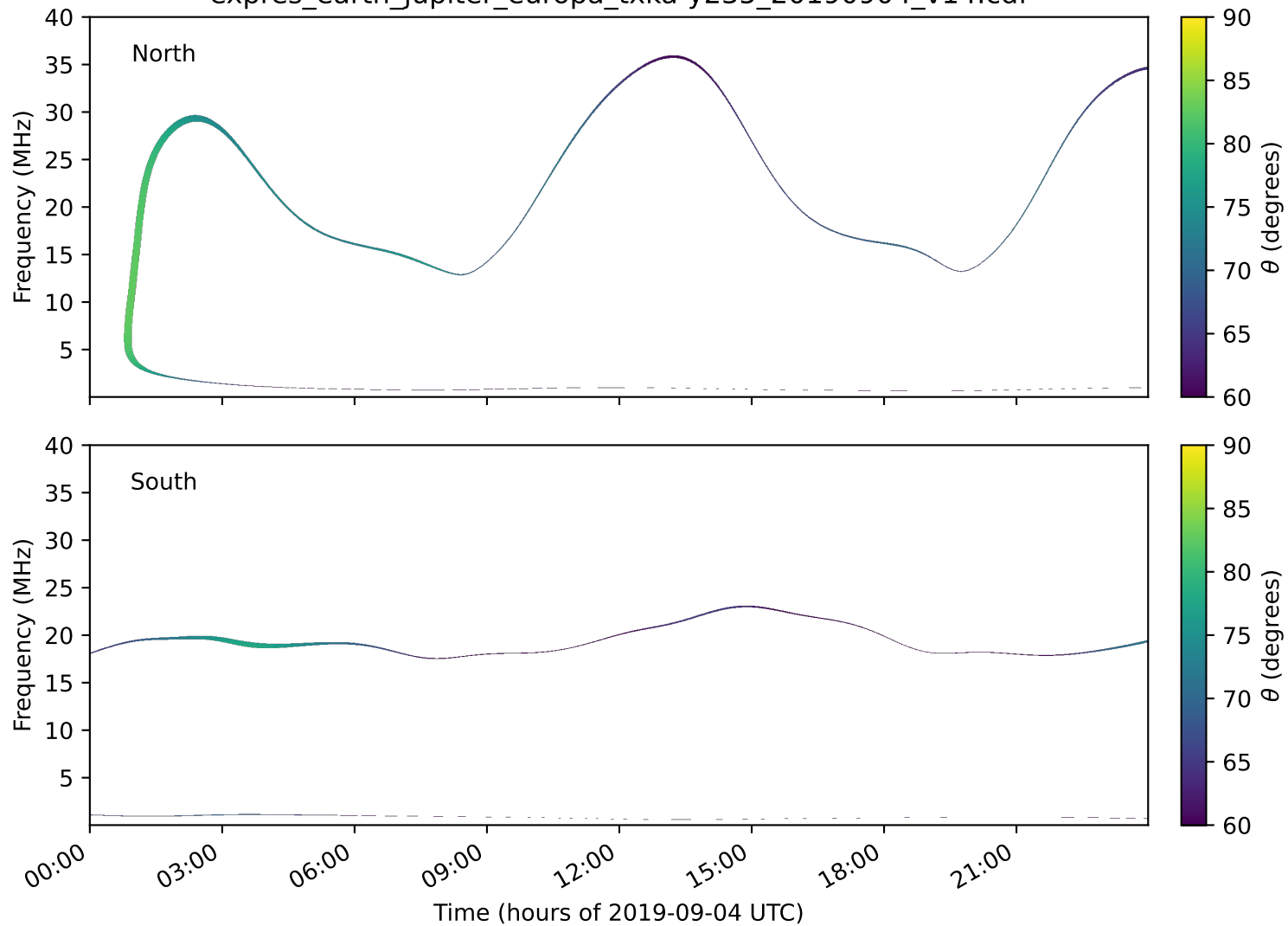
expres_earth_jupiter_europa_txka-y235_20190904_v14.cdf
