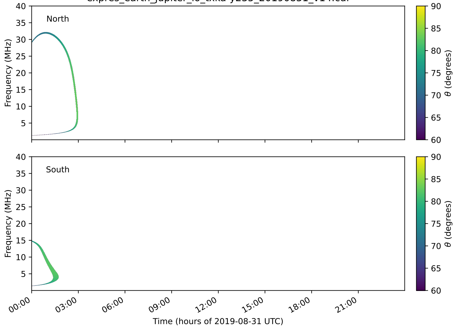
expres_earth_jupiter_io_txka-y235_20190831_v14.cdf
