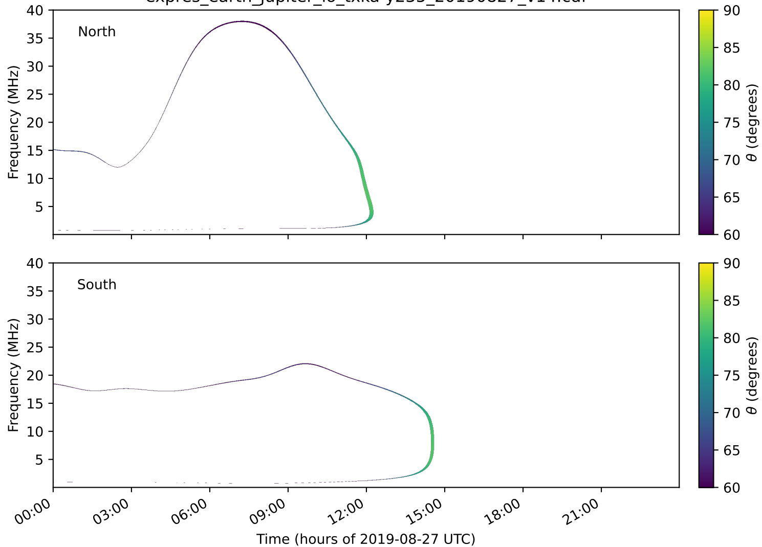
expres_earth_jupiter_io_txka-y235_20190827_v14.cdf
