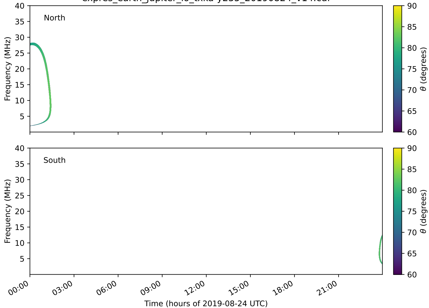
expres_earth_jupiter_io_txka-y235_20190824_v14.cdf
