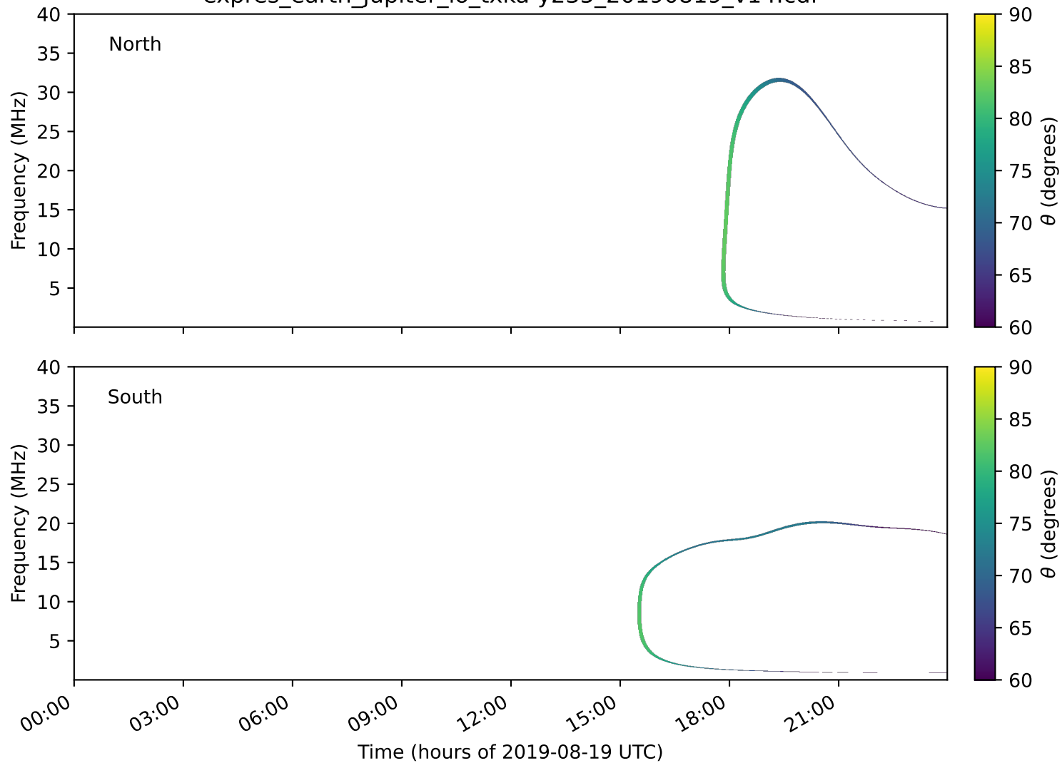
expres_earth_jupiter_io_txka-y235_20190819_v14.cdf
