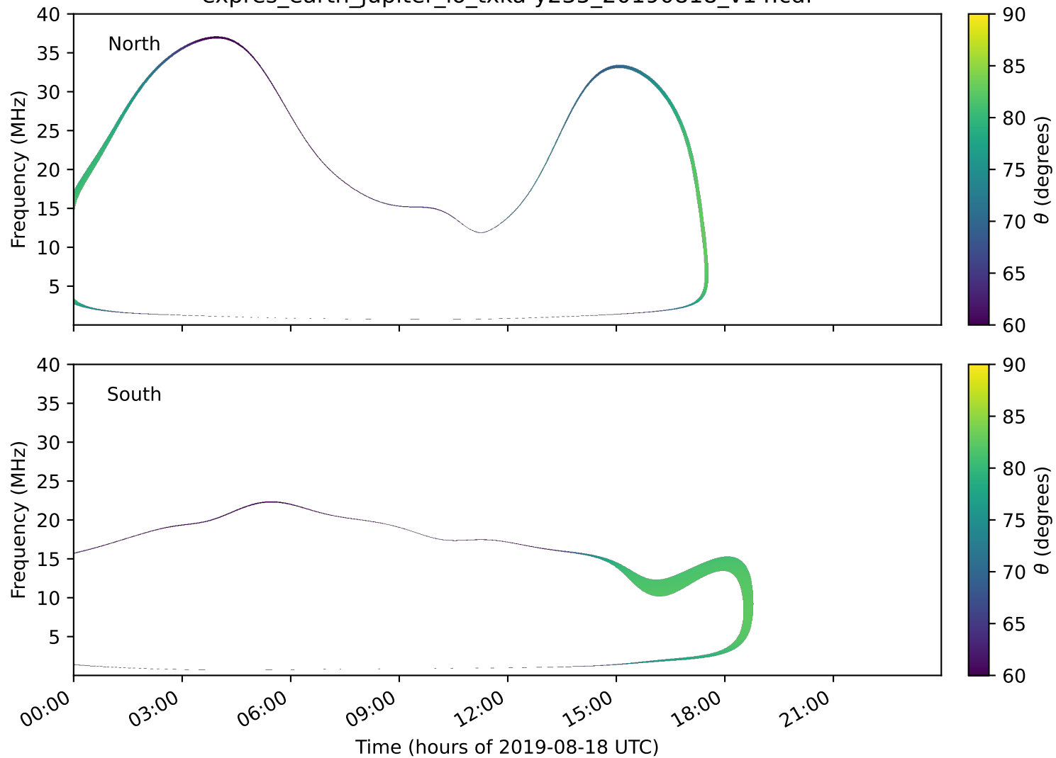
expres_earth_jupiter_io_txka-y235_20190818_v14.cdf
