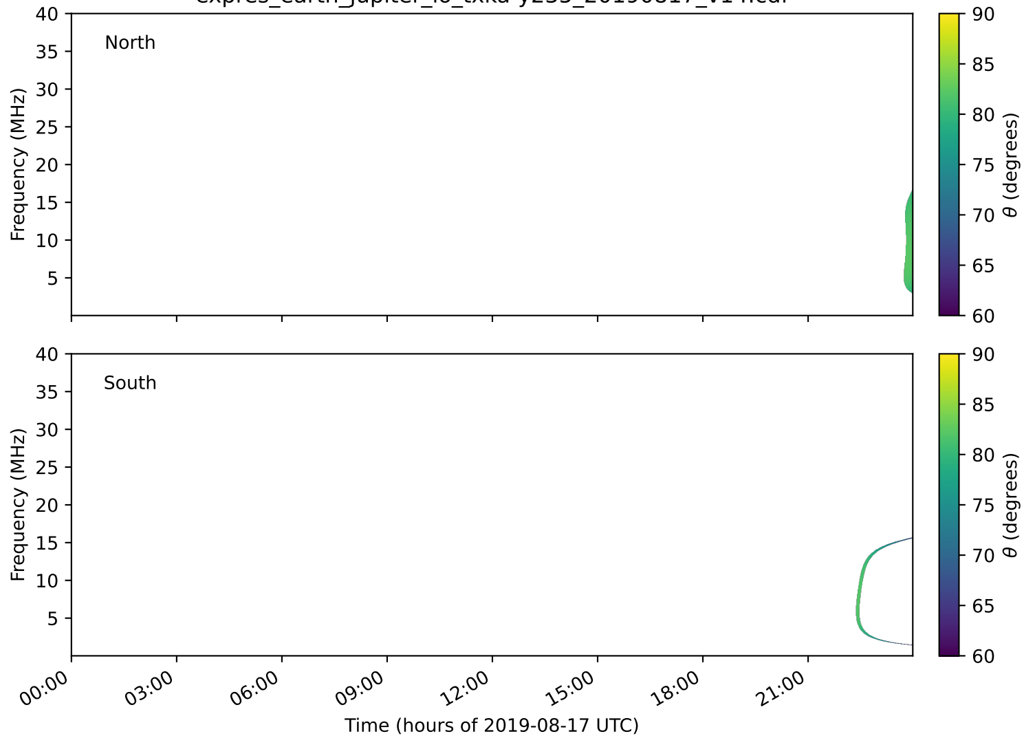
expres_earth_jupiter_io_txka-y235_20190817_v14.cdf
