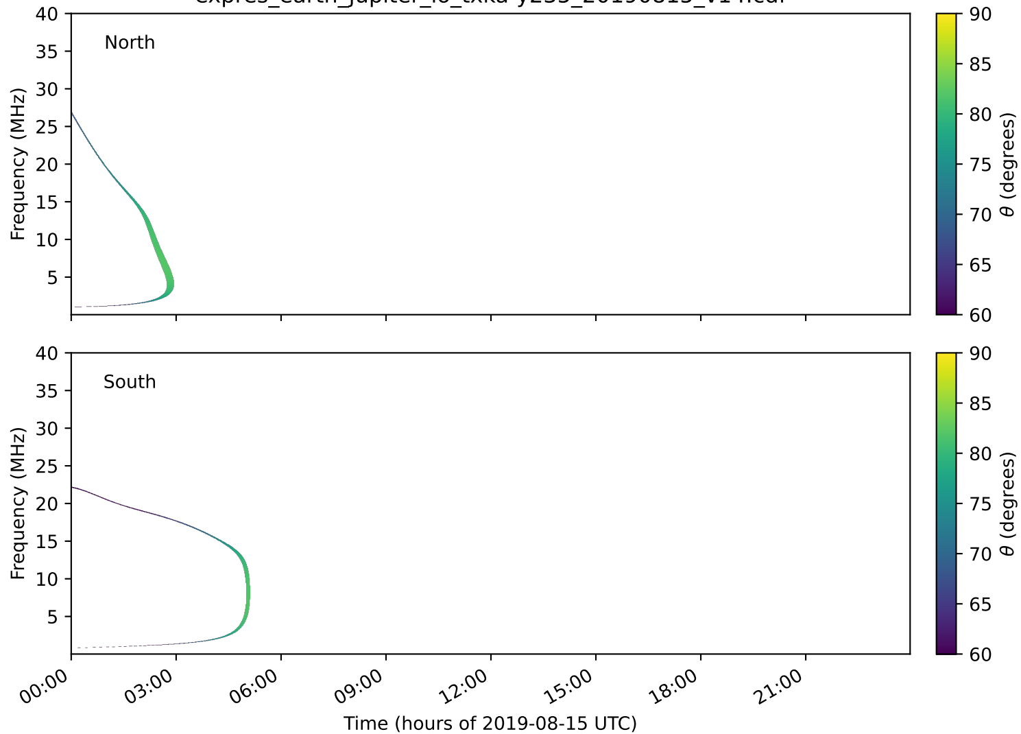
expres_earth_jupiter_io_txka-y235_20190815_v14.cdf
