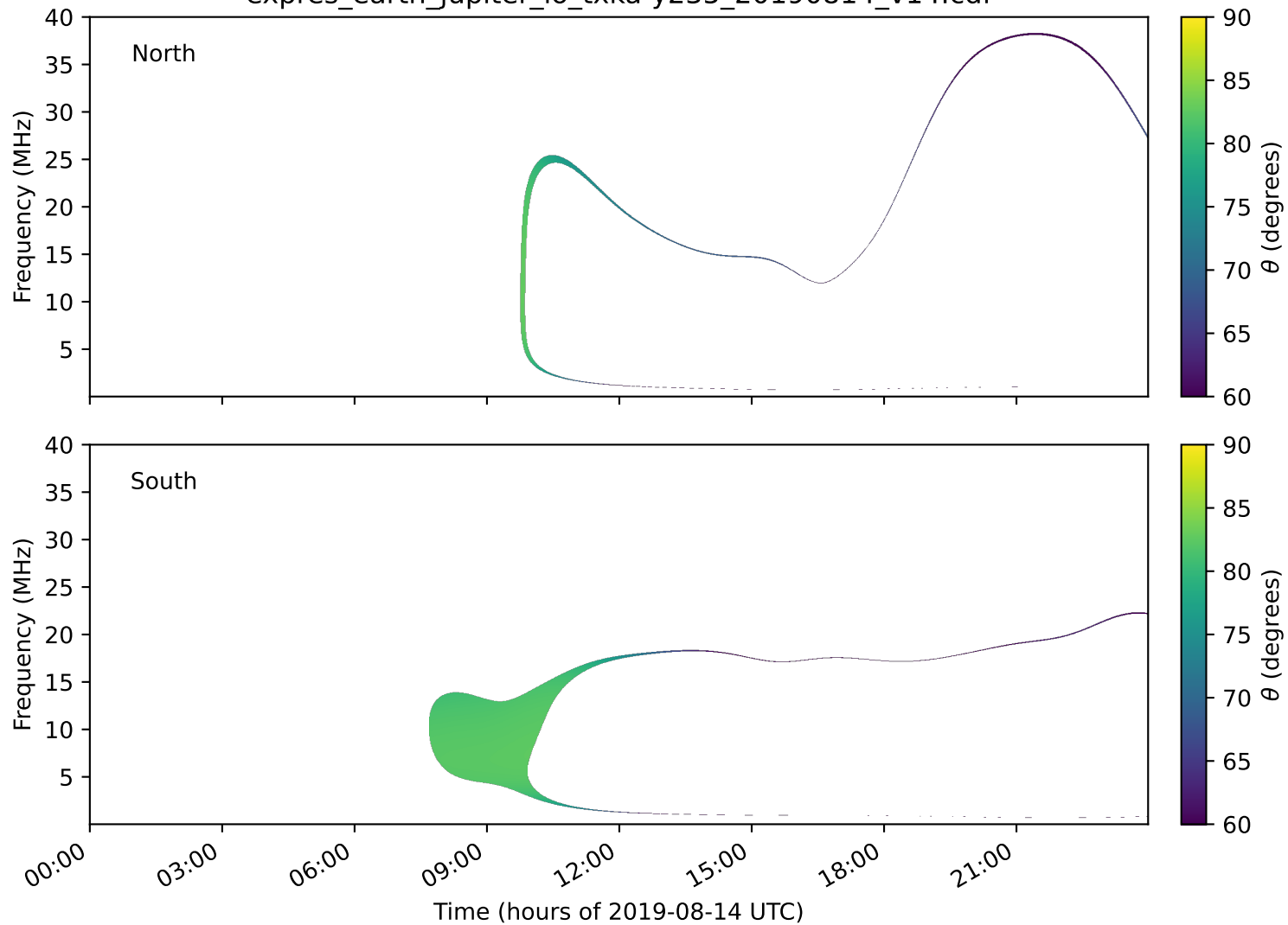
expres_earth_jupiter_io_txka-y235_20190814_v14.cdf
