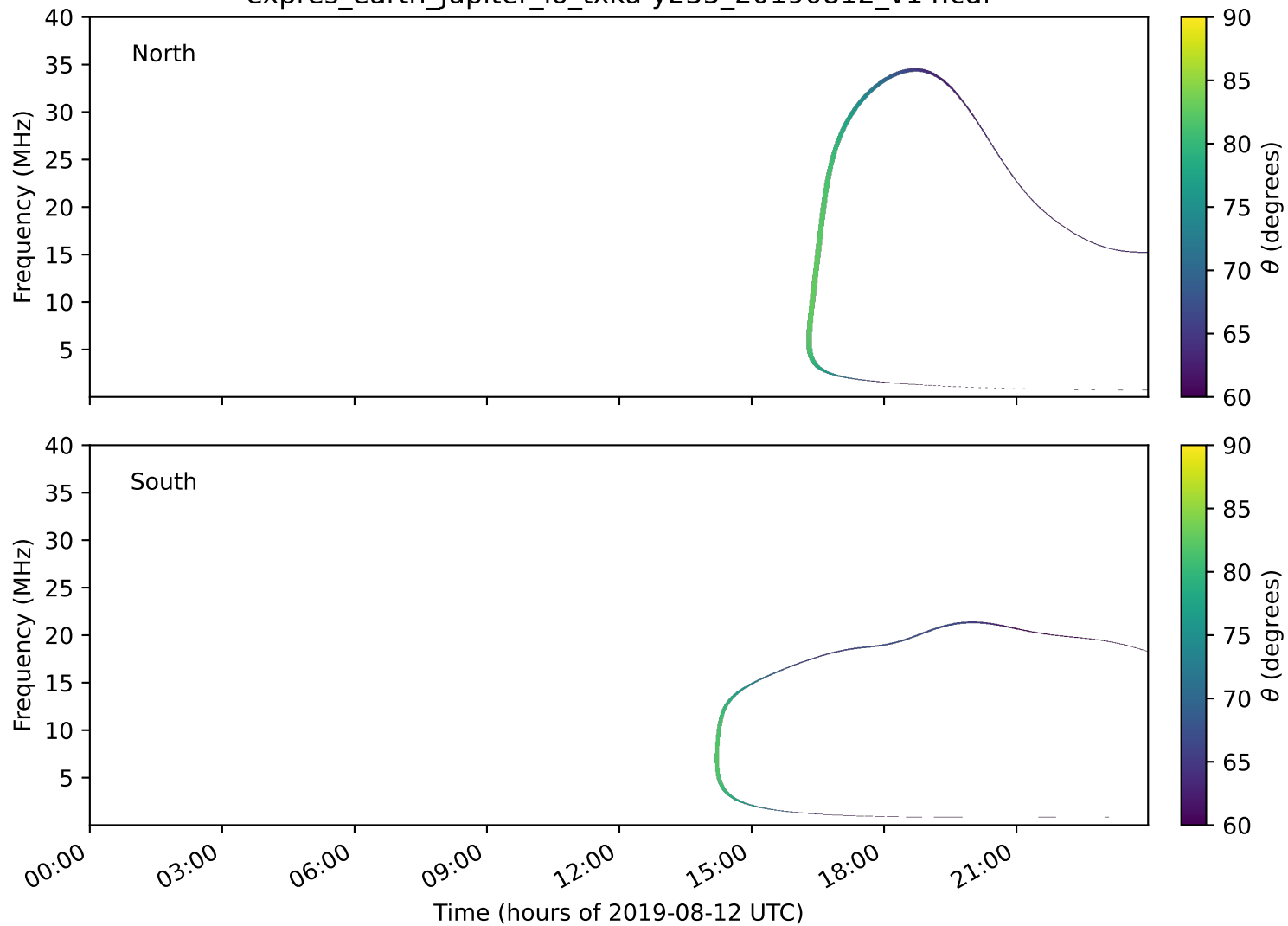
expres_earth_jupiter_io_txka-y235_20190812_v14.cdf
