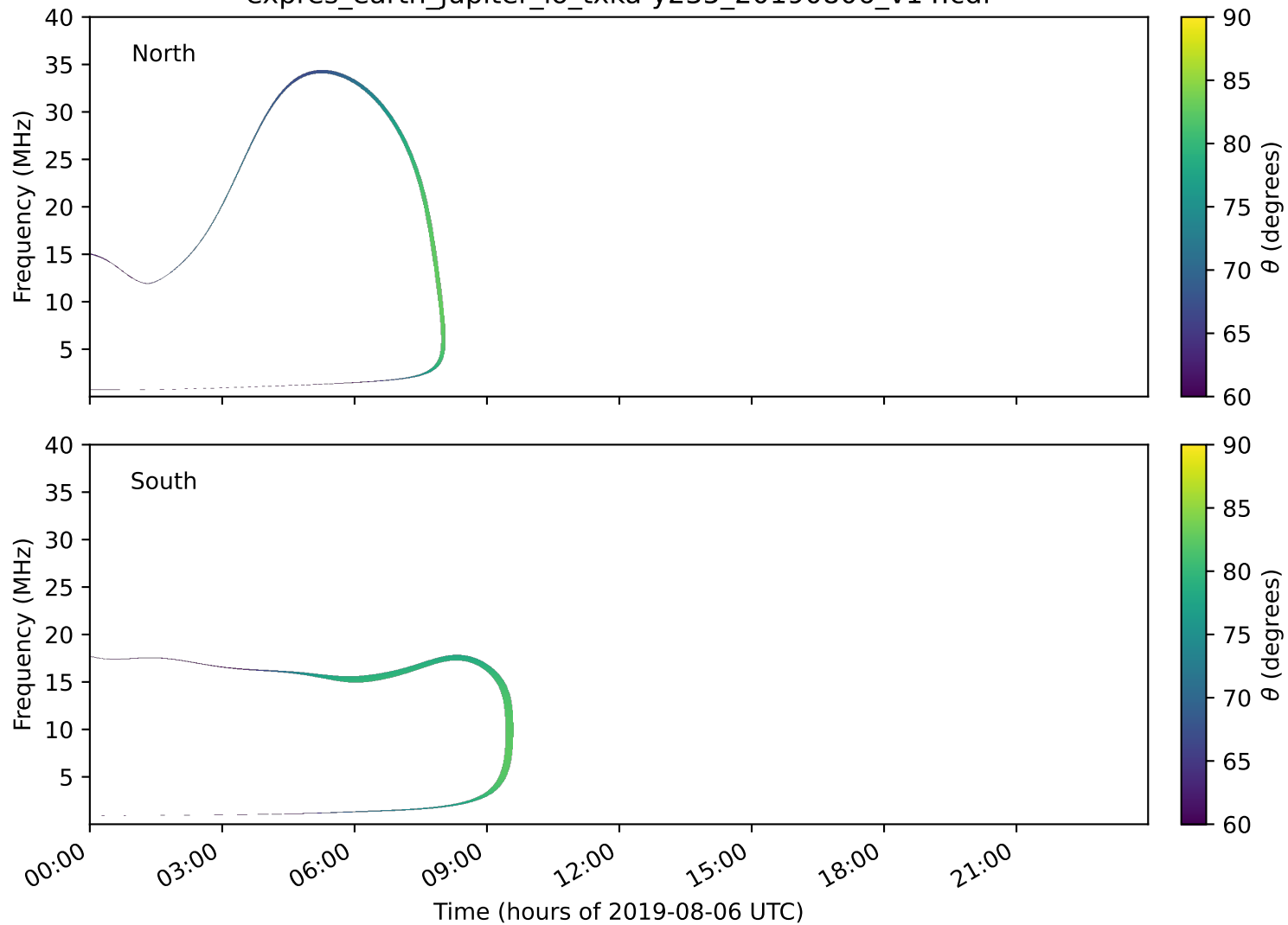
expres_earth_jupiter_io_txka-y235_20190806_v14.cdf
