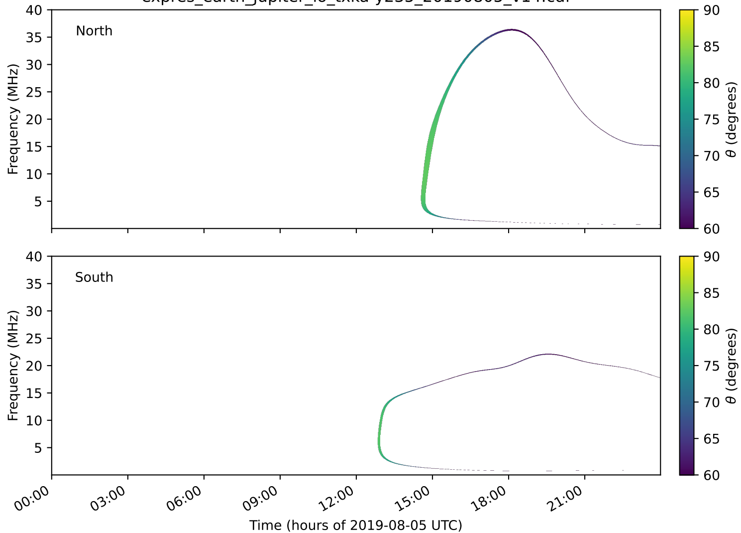
expres_earth_jupiter_io_txka-y235_20190805_v14.cdf
