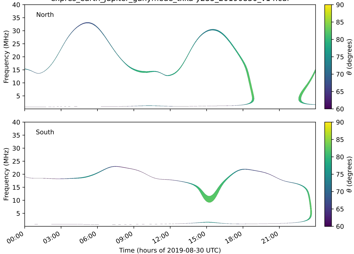
expres_earth_jupiter_ganymede_txka-y235_20190830_v14.cdf
