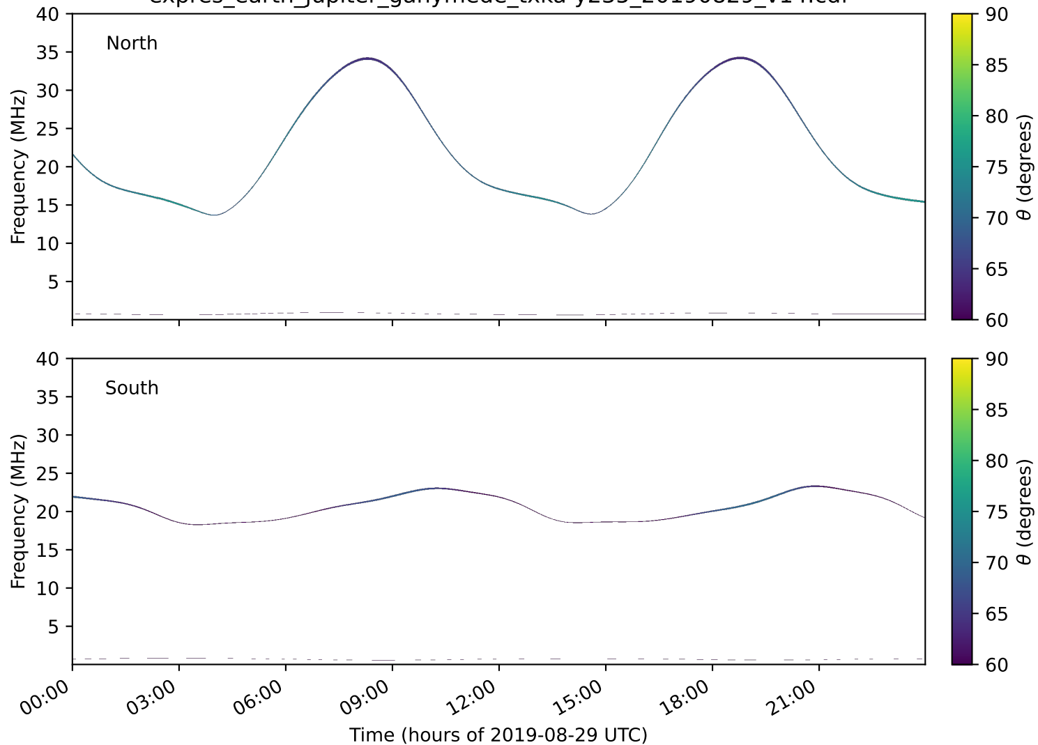
expres_earth_jupiter_ganymede_txka-y235_20190829_v14.cdf
