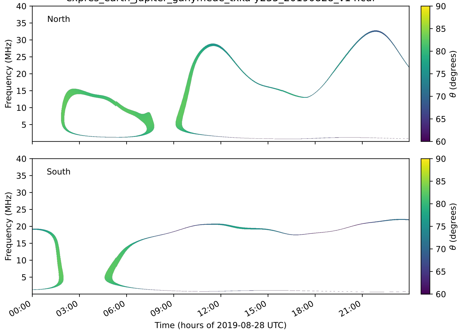
expres_earth_jupiter_ganymede_txka-y235_20190828_v14.cdf
