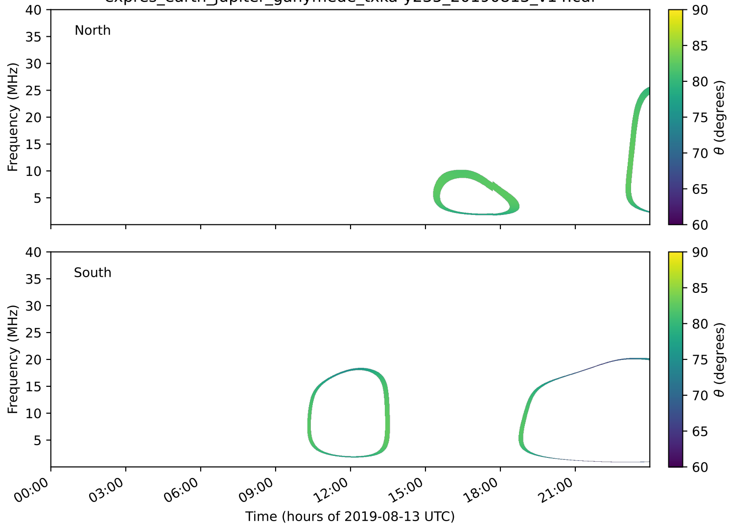
expres_earth_jupiter_ganymede_txka-y235_20190813_v14.cdf
