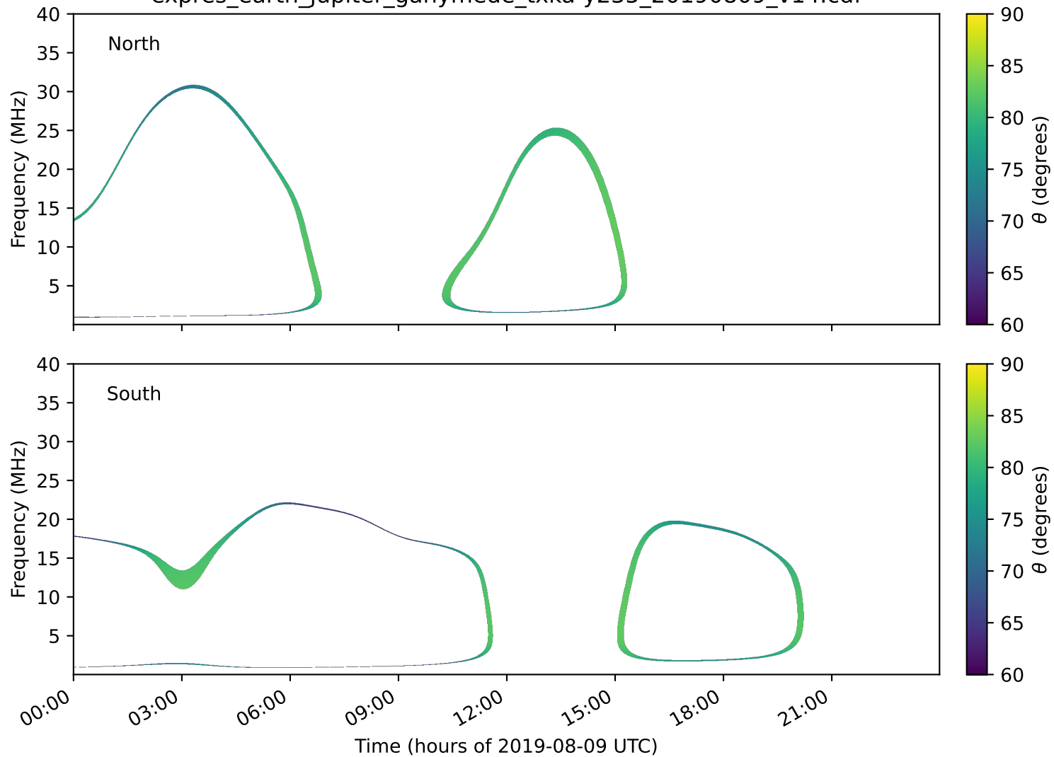
expres_earth_jupiter_ganymede_txka-y235_20190809_v14.cdf
