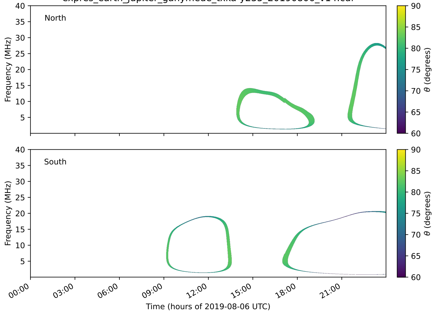
expres_earth_jupiter_ganymede_txka-y235_20190806_v14.cdf
