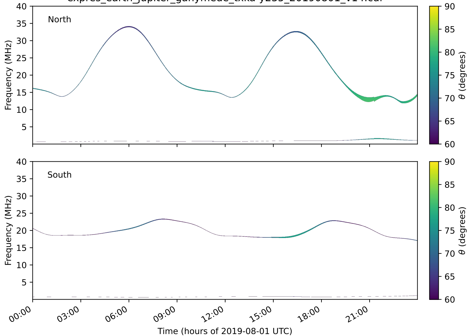
expres_earth_jupiter_ganymede_txka-y235_20190801_v14.cdf
