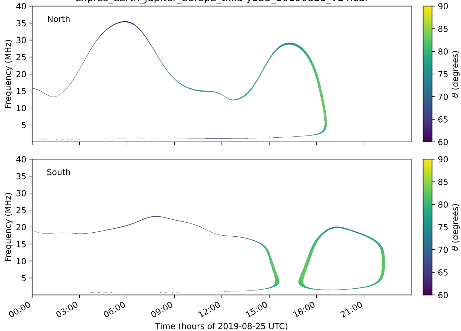
expres_earth_jupiter_europa_txka-y235_20190825_v14.cdf
