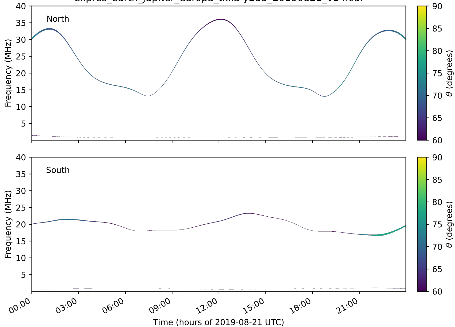
expres_earth_jupiter_europa_txka-y235_20190821_v14.cdf
