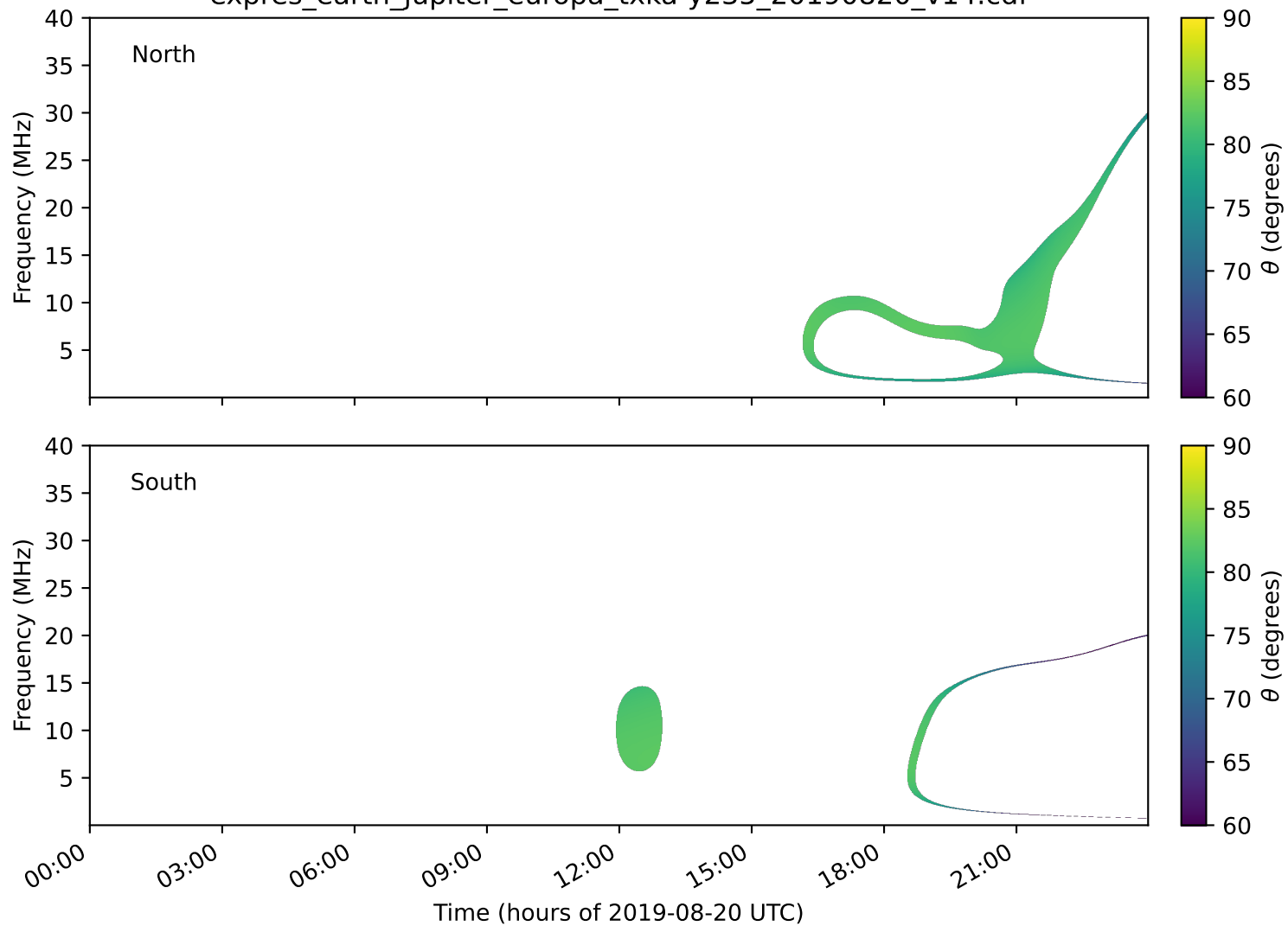
expres_earth_jupiter_europa_txka-y235_20190820_v14.cdf
