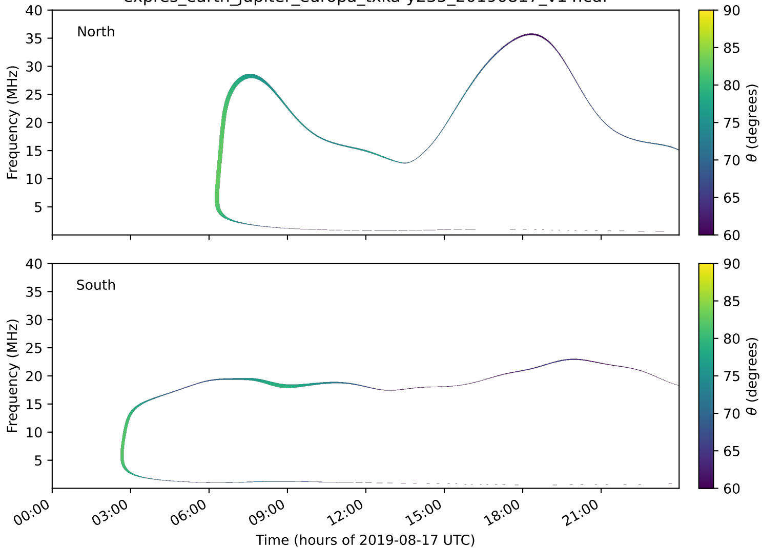
expres_earth_jupiter_europa_txka-y235_20190817_v14.cdf
