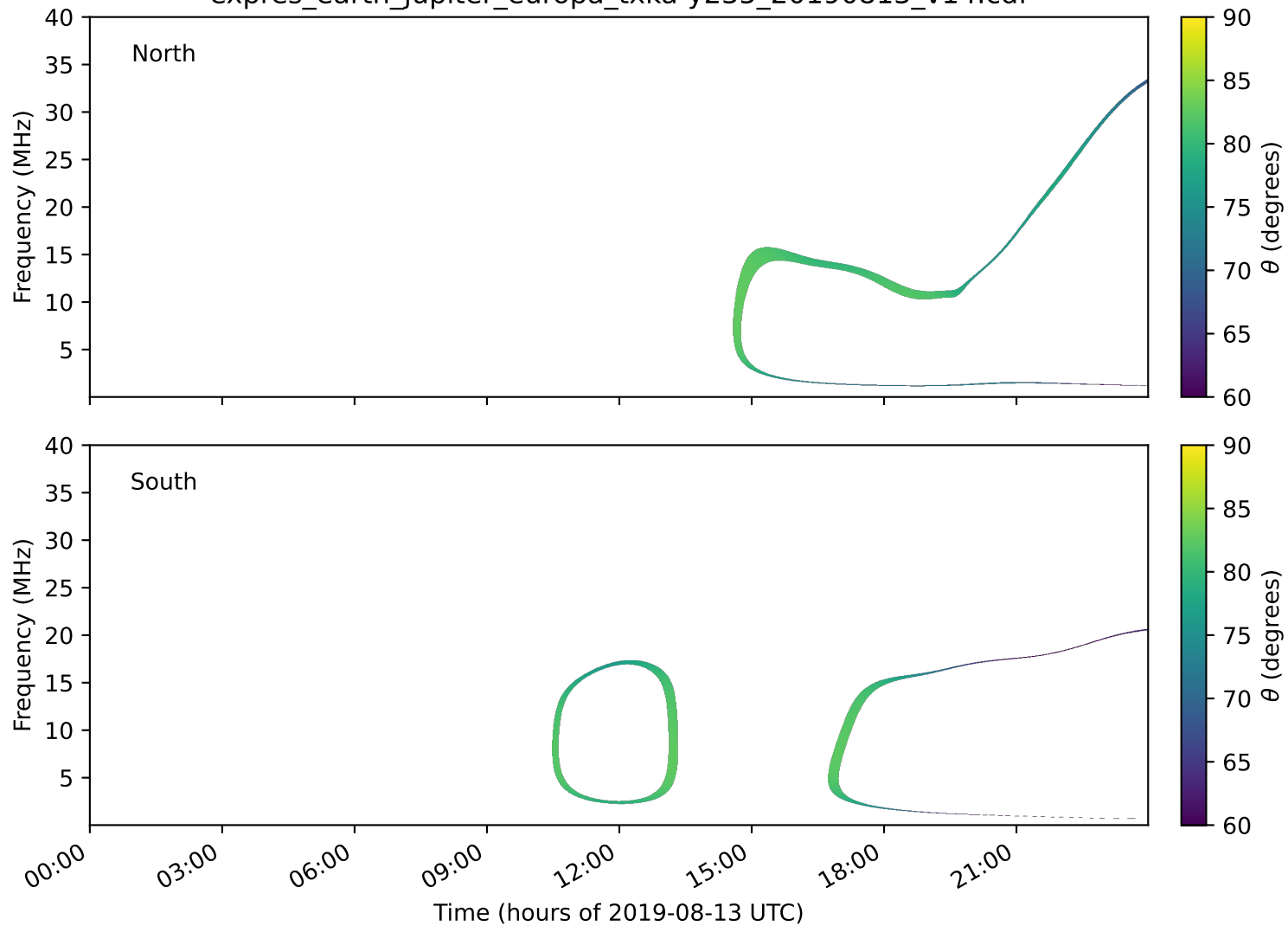
expres_earth_jupiter_europa_txka-y235_20190813_v14.cdf
