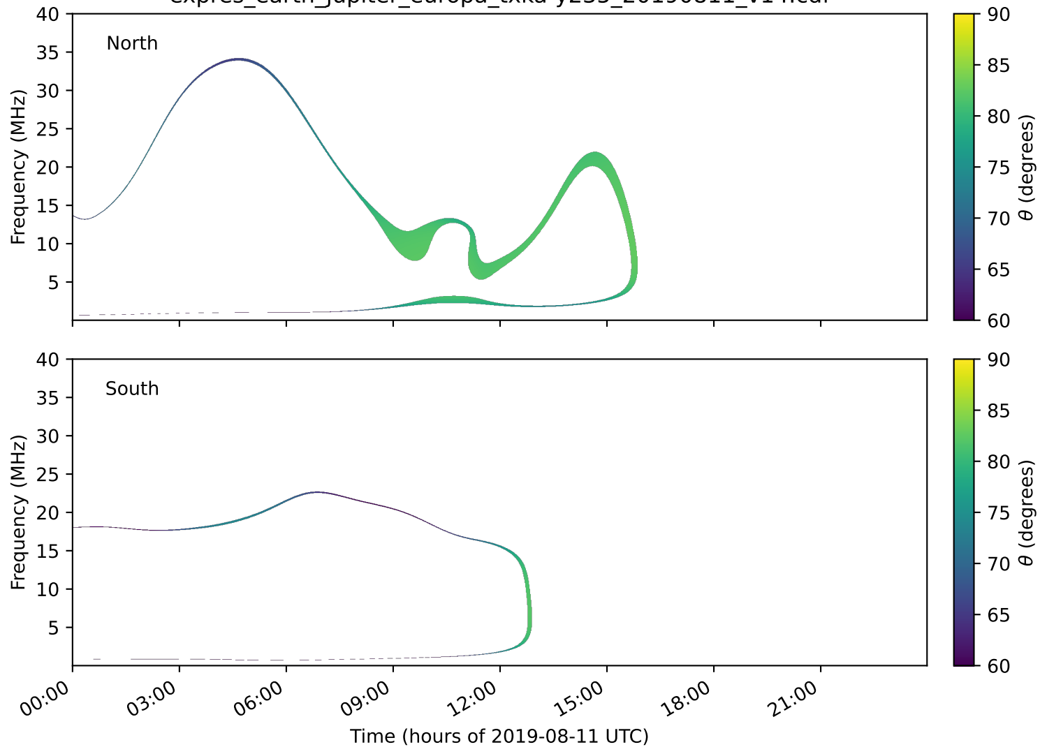
expres_earth_jupiter_europa_txka-y235_20190811_v14.cdf
