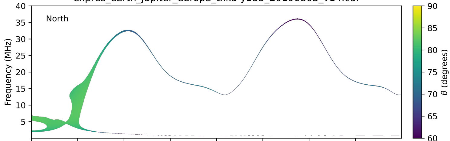
expres_earth_jupiter_europa_txka-y235_20190803_v14.cdf
