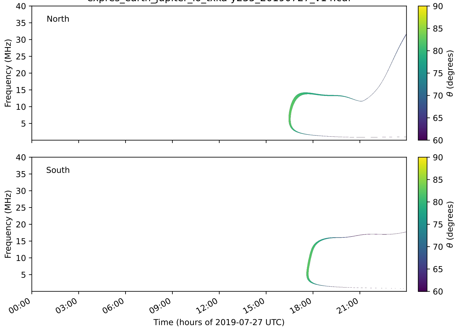
expres_earth_jupiter_io_txka-y235_20190727_v14.cdf
