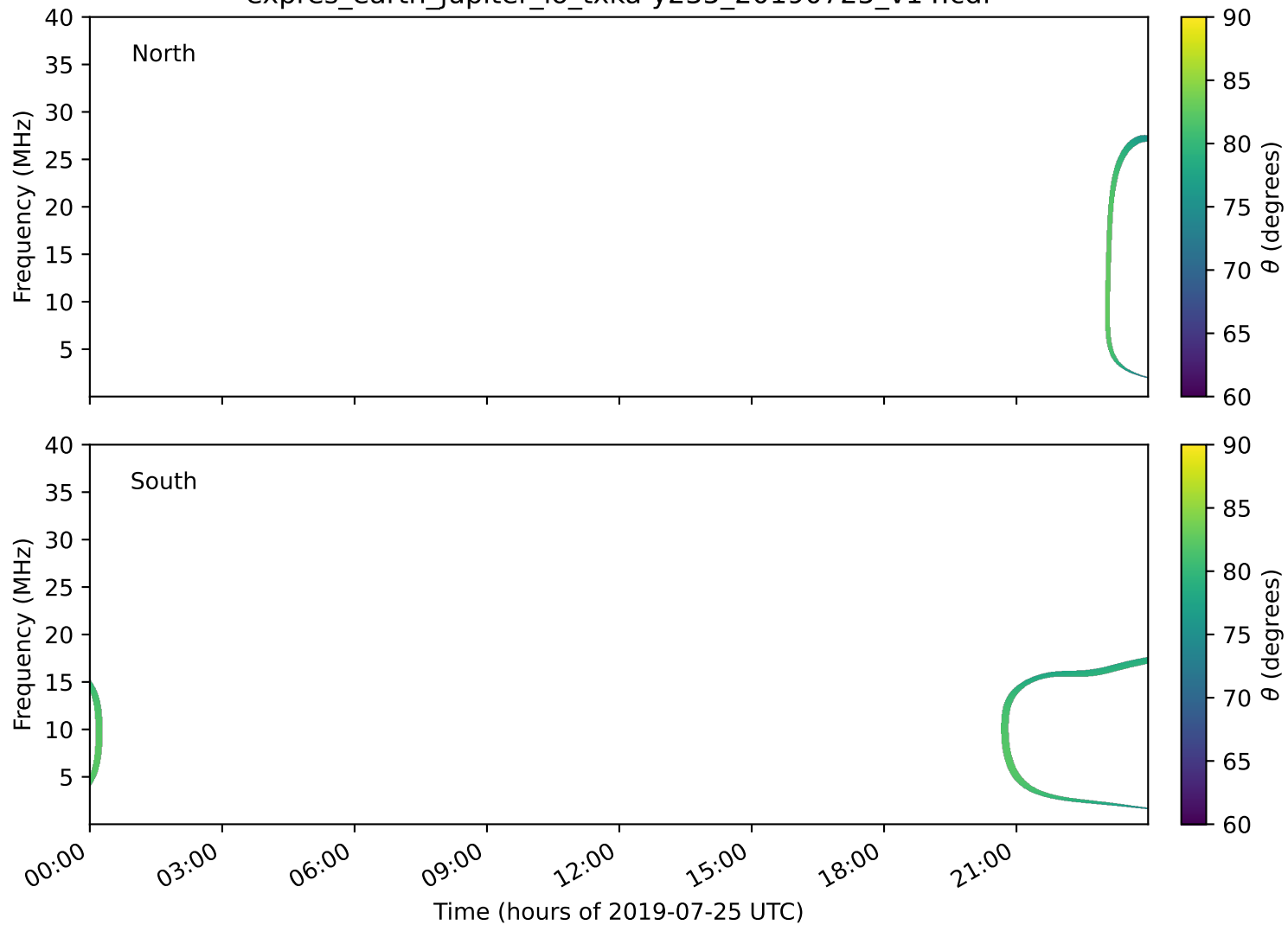
expres_earth_jupiter_io_txka-y235_20190725_v14.cdf
