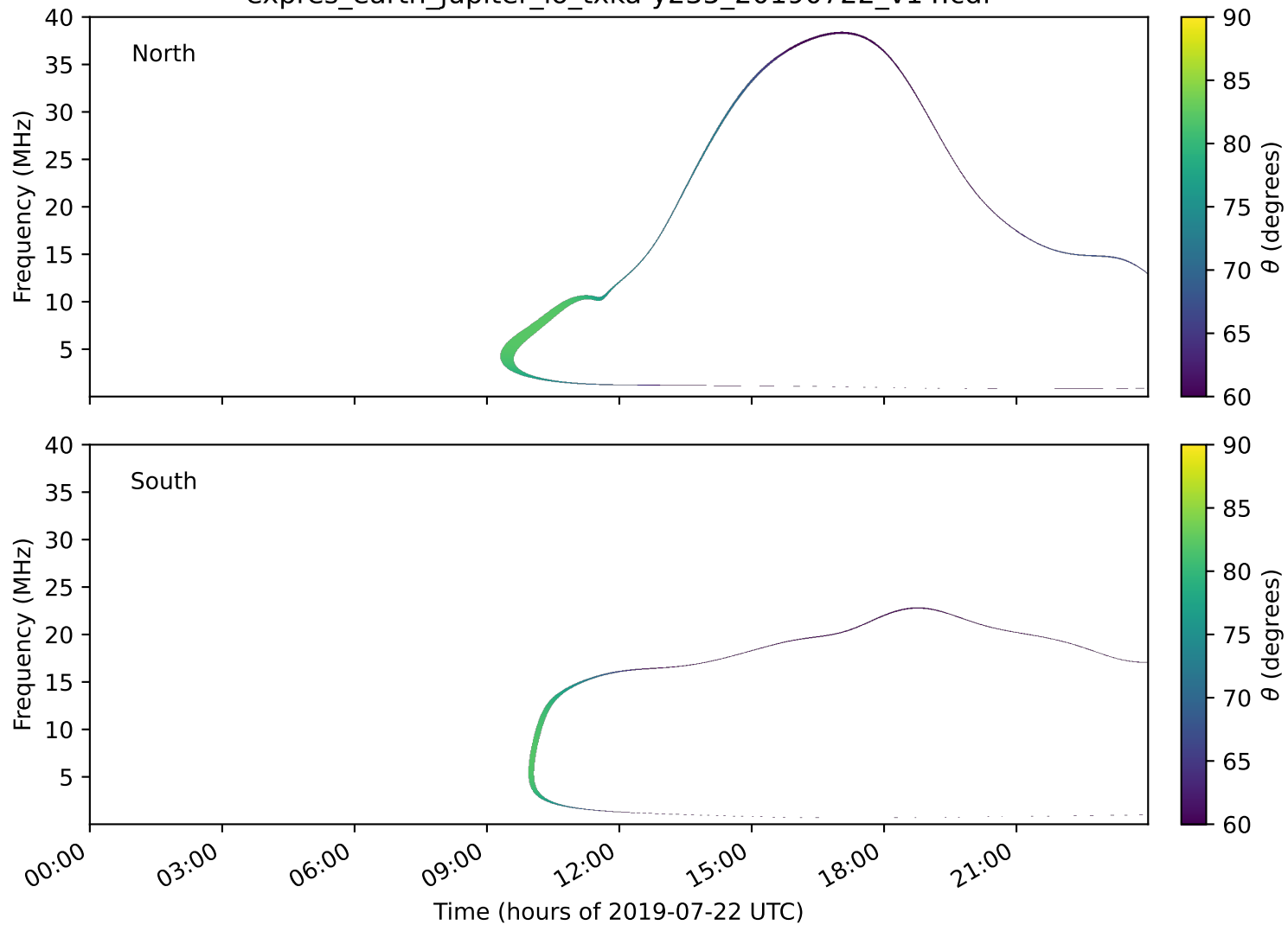
expres_earth_jupiter_io_txka-y235_20190722_v14.cdf
