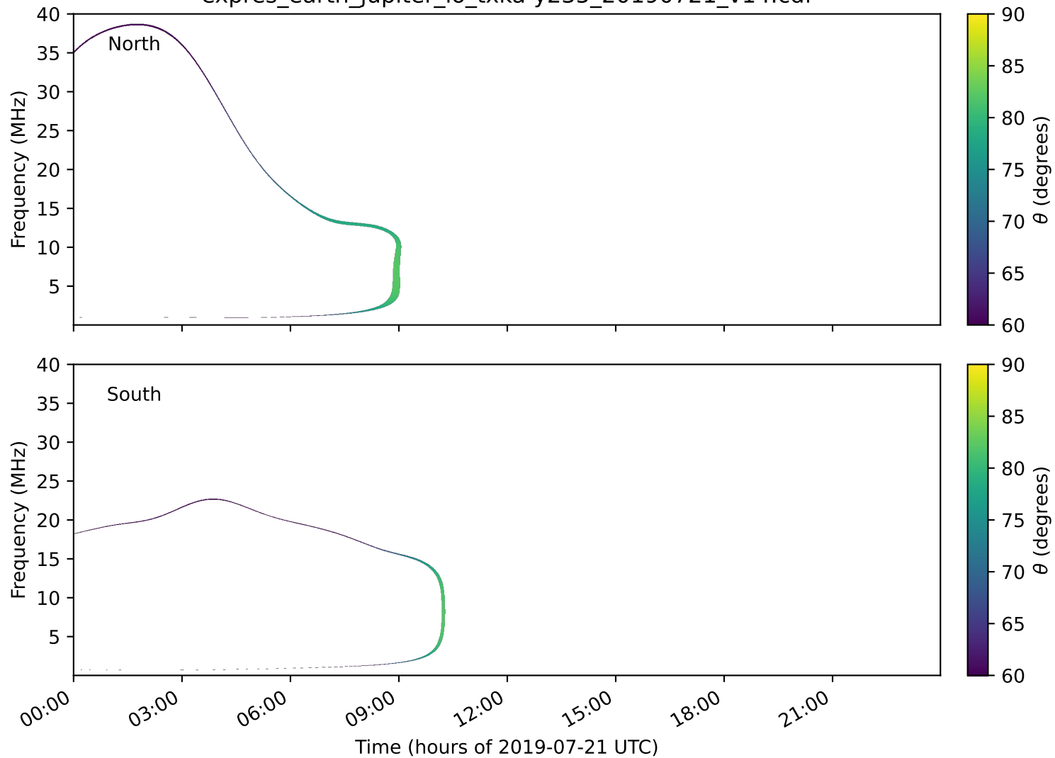
expres_earth_jupiter_io_txka-y235_20190721_v14.cdf
