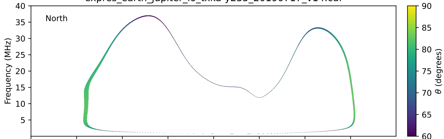
expres_earth_jupiter_io_txka-y235_20190717_v14.cdf
