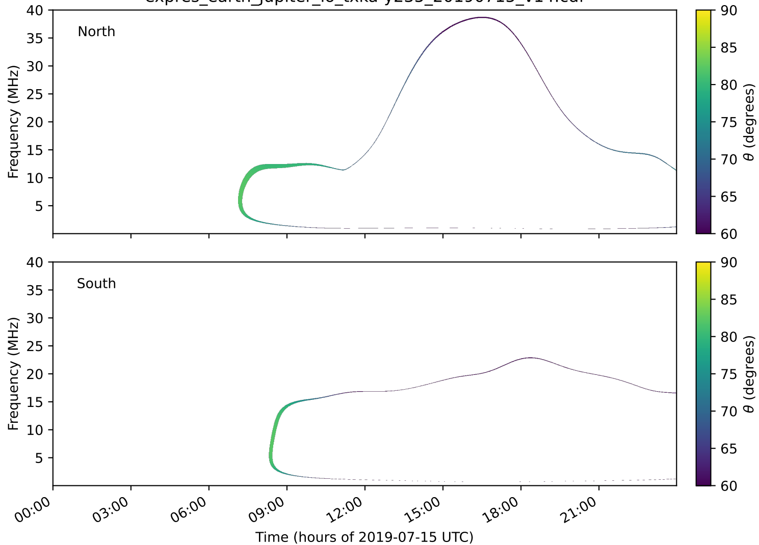
expres_earth_jupiter_io_txka-y235_20190715_v14.cdf
