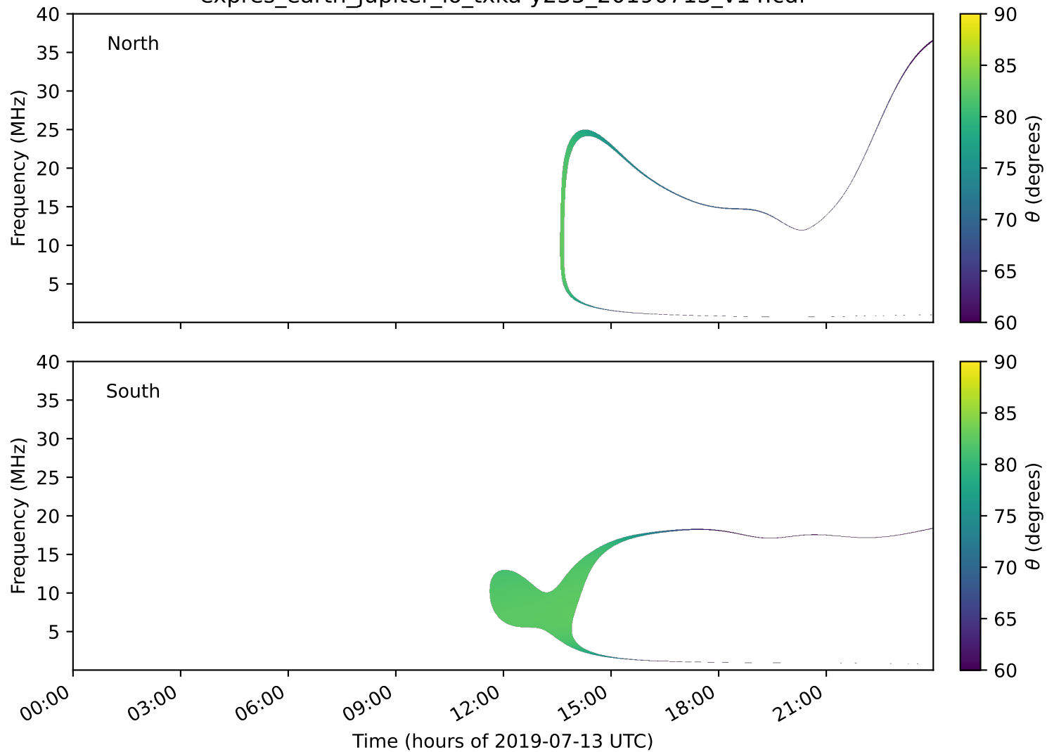
expres_earth_jupiter_io_txka-y235_20190713_v14.cdf
