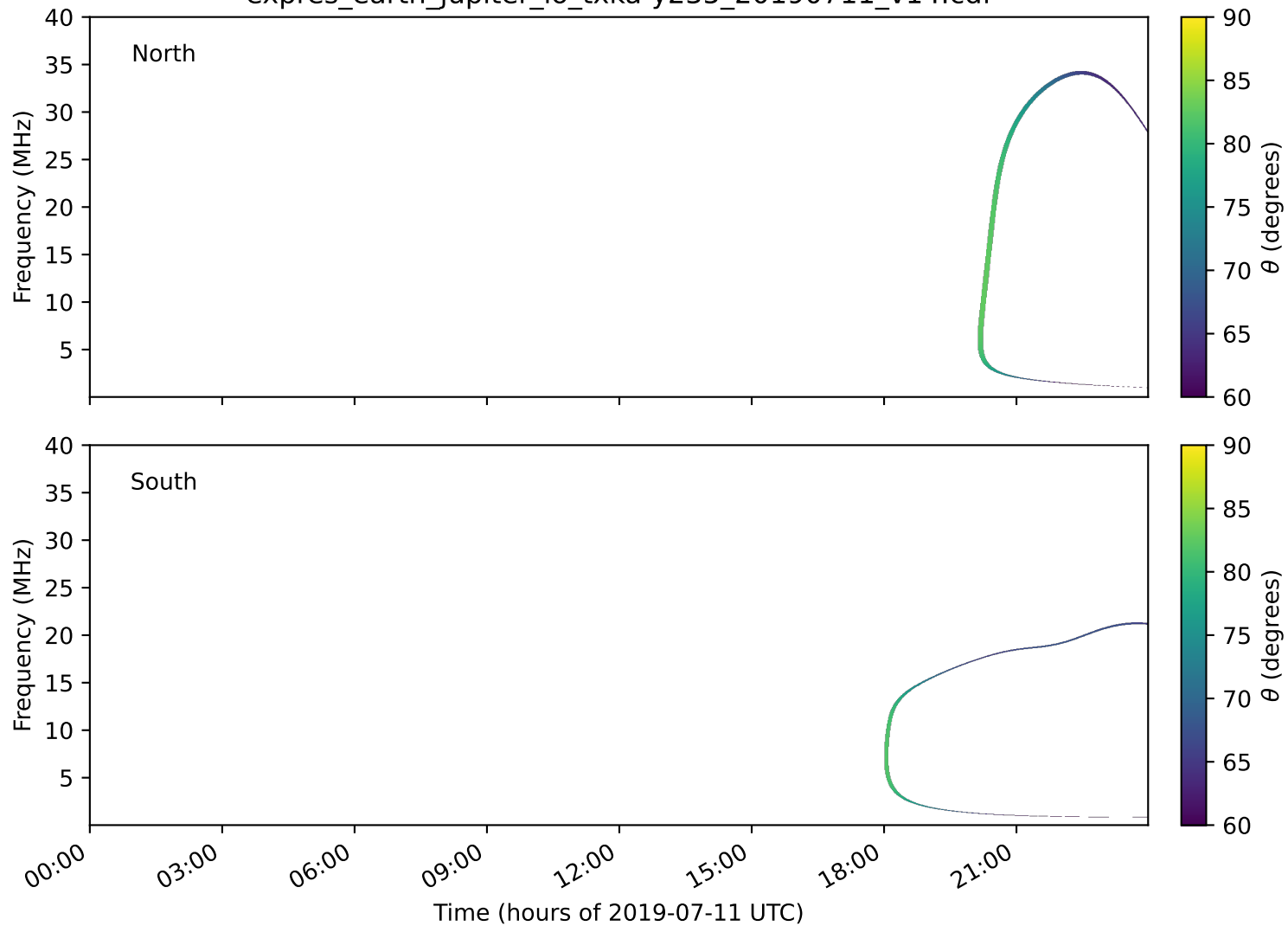
expres_earth_jupiter_io_txka-y235_20190711_v14.cdf
