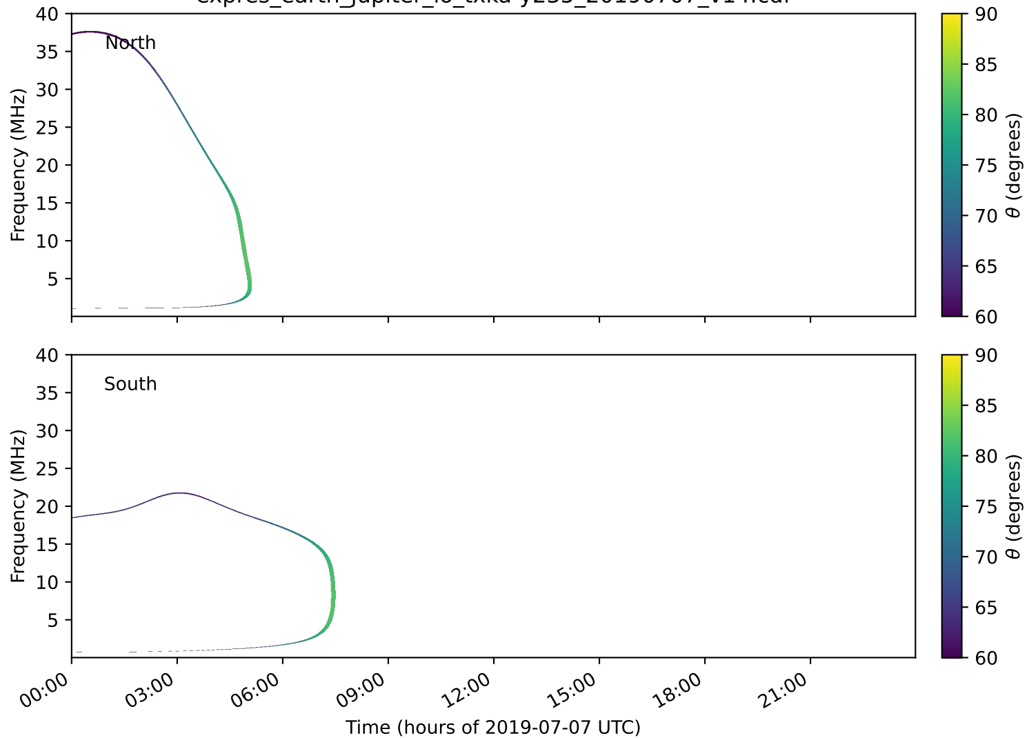
expres_earth_jupiter_io_txka-y235_20190707_v14.cdf
