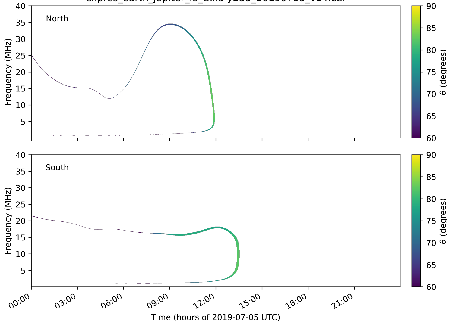
expres_earth_jupiter_io_txka-y235_20190705_v14.cdf
