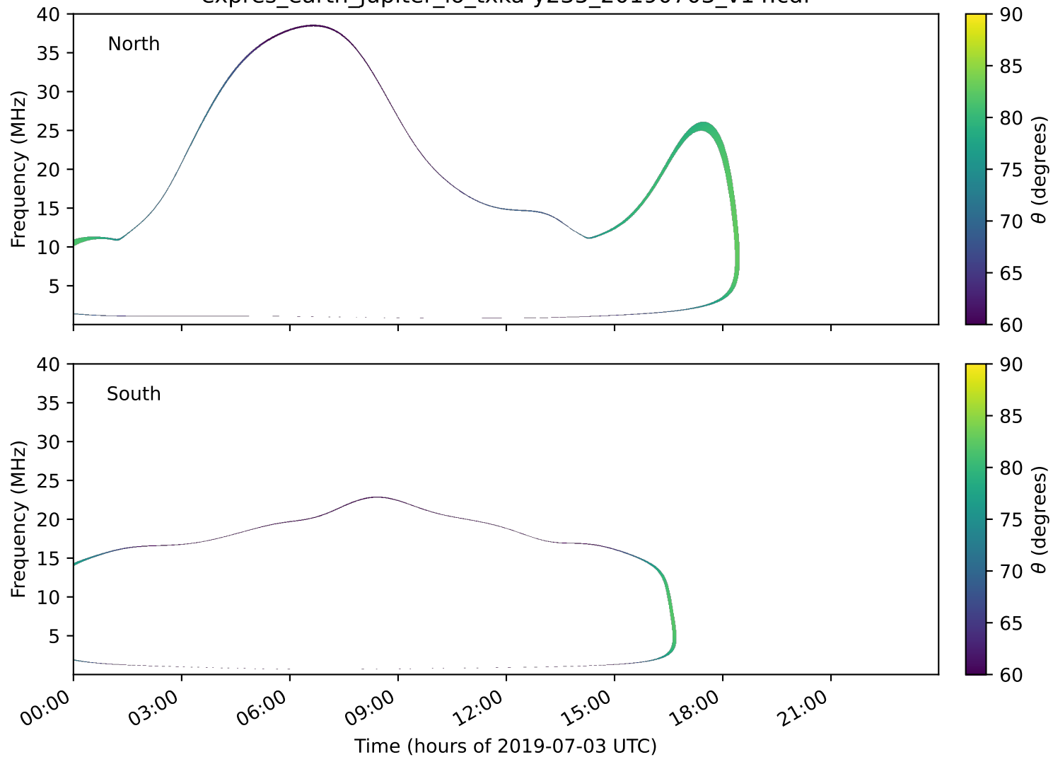
expres_earth_jupiter_io_txka-y235_20190703_v14.cdf
