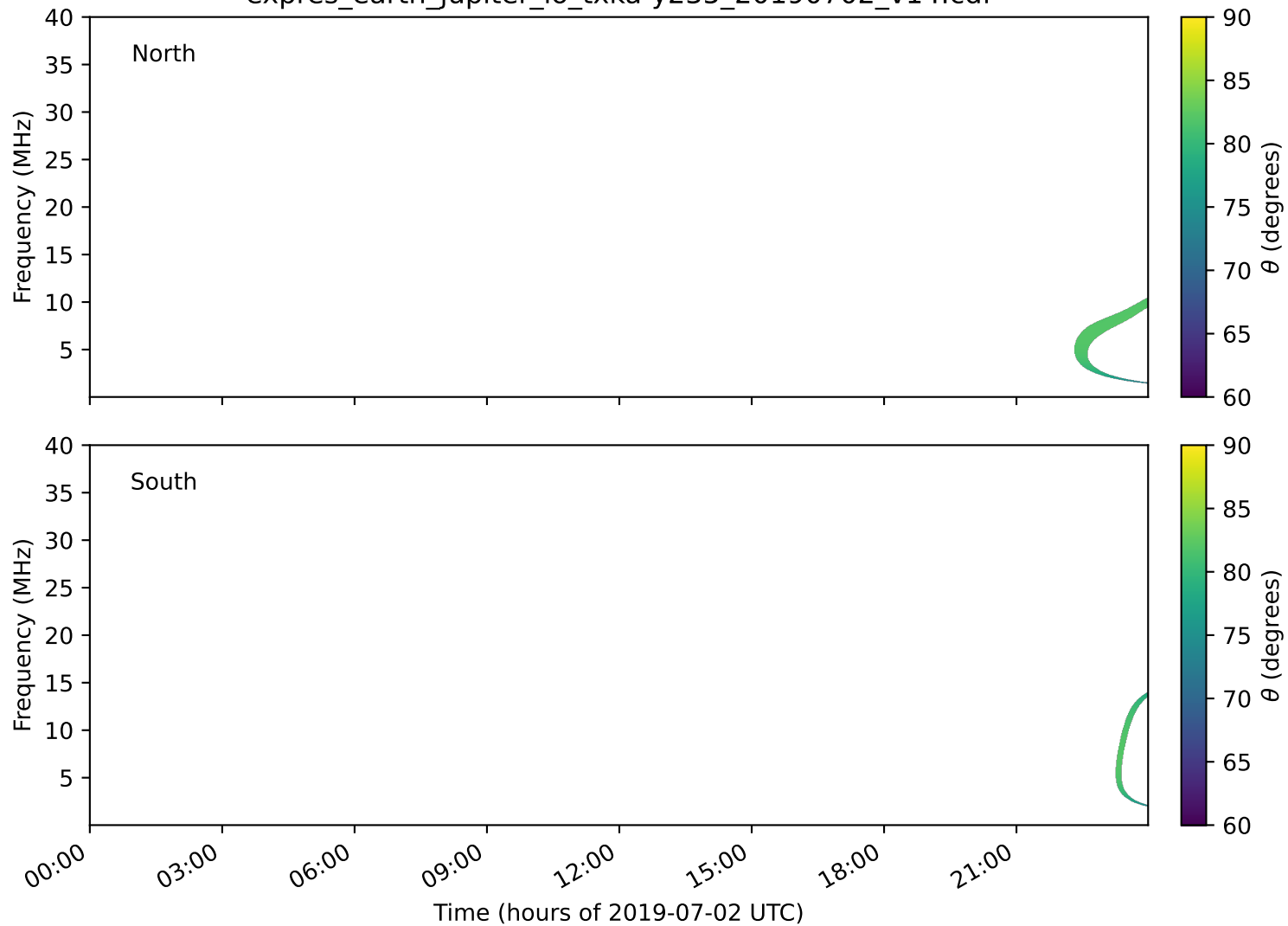
expres_earth_jupiter_io_txka-y235_20190702_v14.cdf
