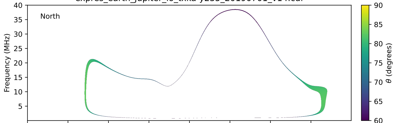
expres_earth_jupiter_io_txka-y235_20190701_v14.cdf
