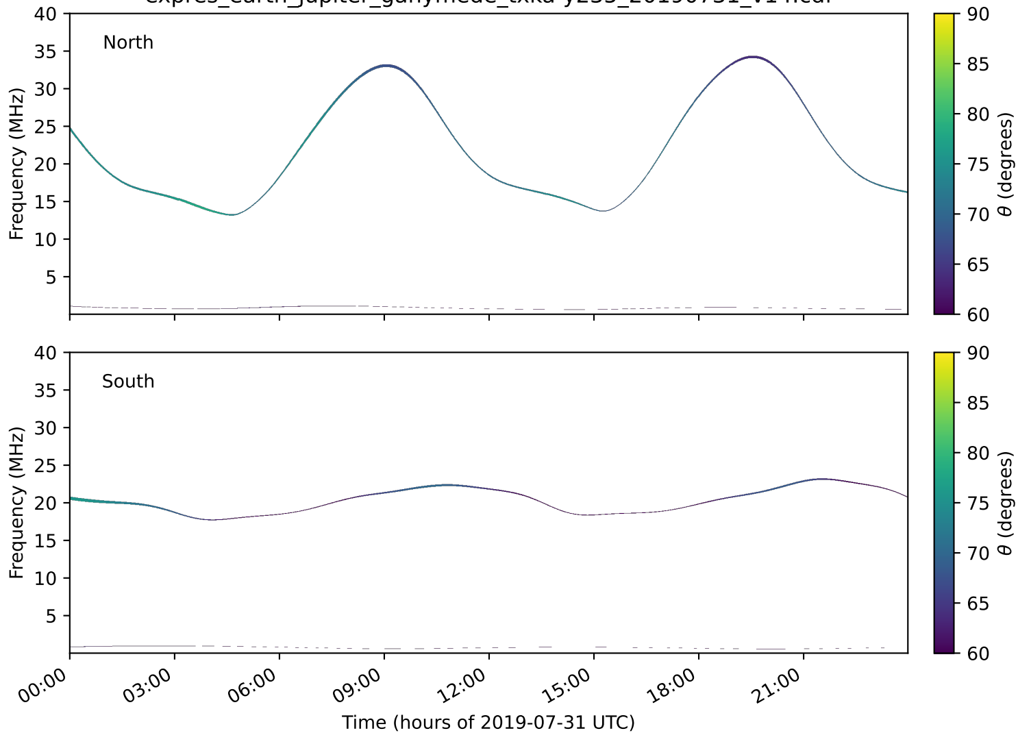
expres_earth_jupiter_ganymede_txka-y235_20190731_v14.cdf
