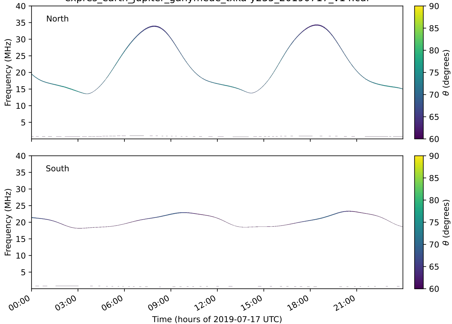
expres_earth_jupiter_ganymede_txka-y235_20190717_v14.cdf
