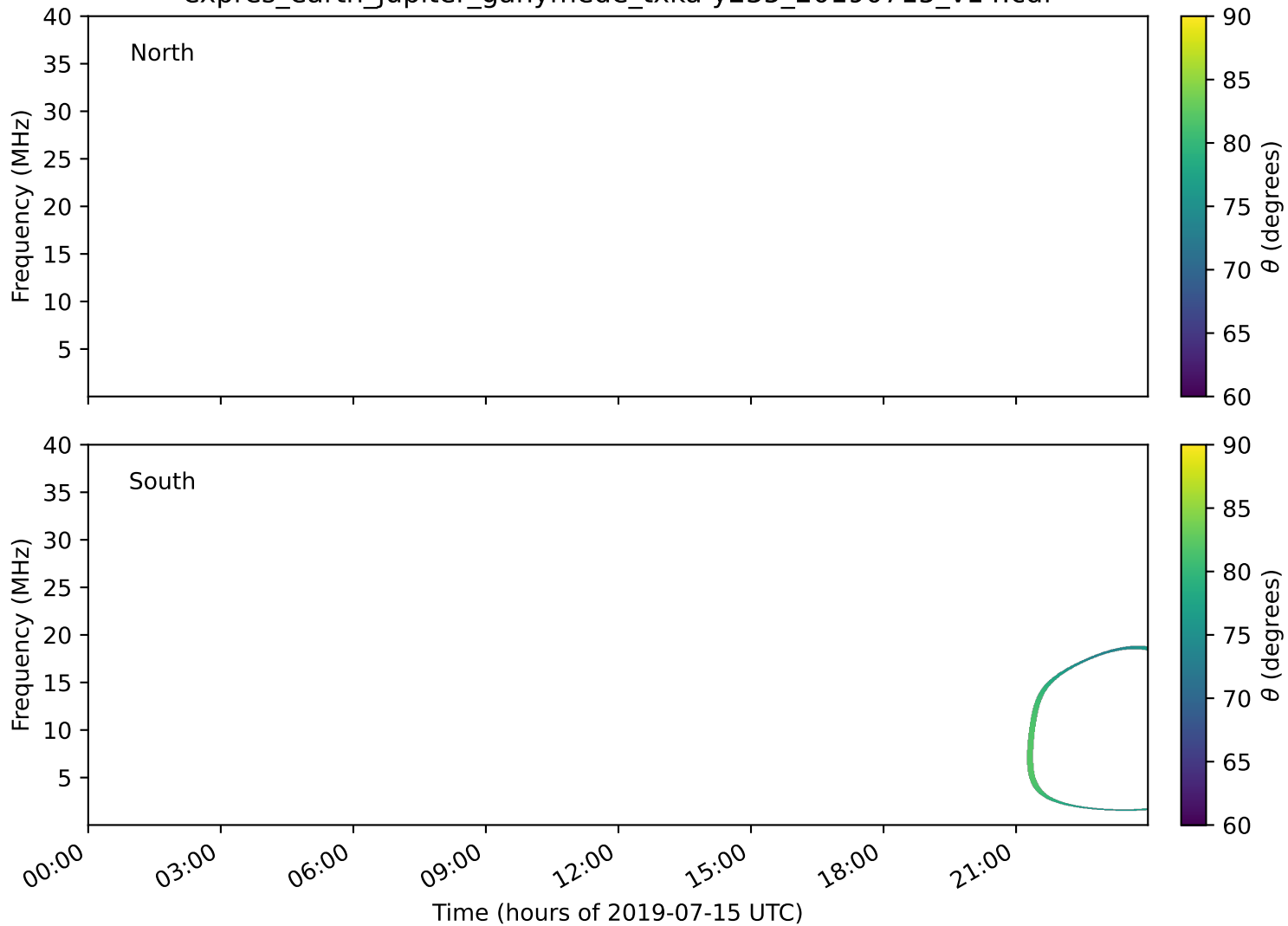
expres_earth_jupiter_ganymede_txka-y235_20190715_v14.cdf
