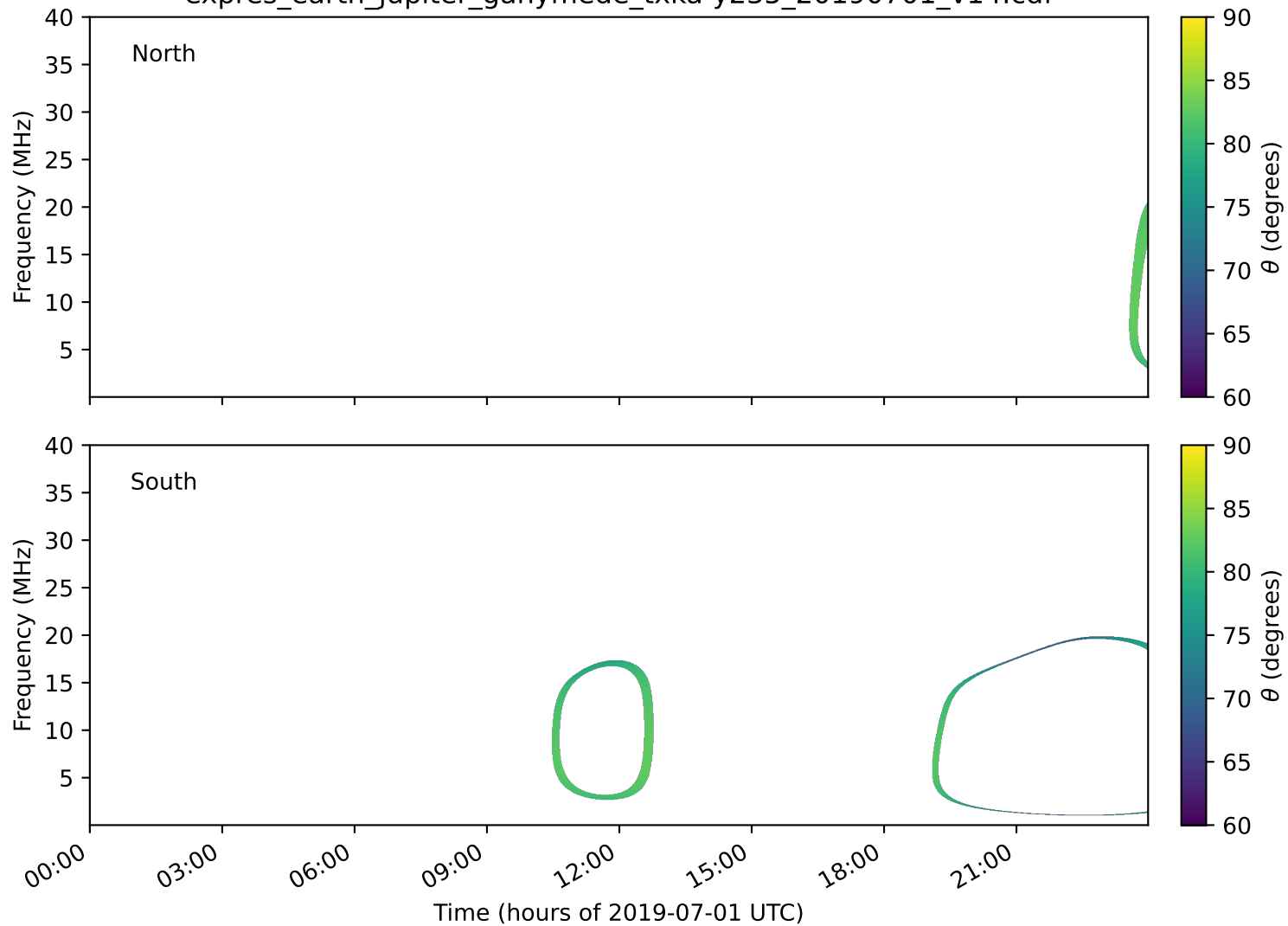
expres_earth_jupiter_ganymede_txka-y235_20190701_v14.cdf
