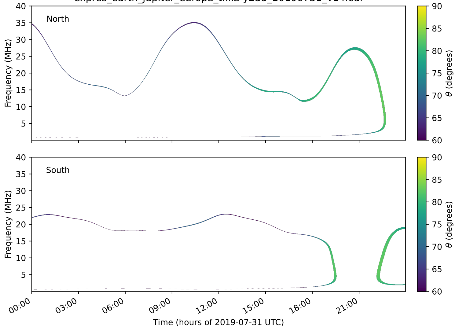
expres_earth_jupiter_europa_txka-y235_20190731_v14.cdf
